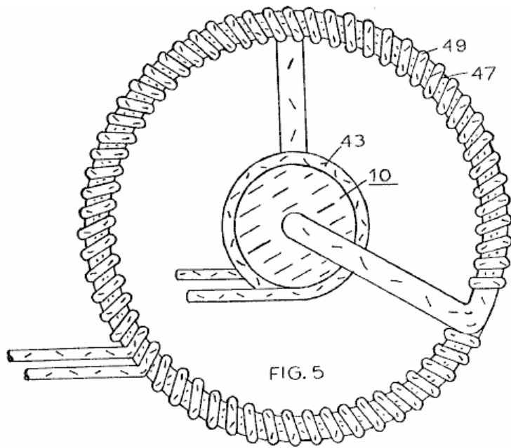
Fig.5 shows a coil arrangement 49, which uses the entire magnetic flux in the closed-loop tubing 47. This is a coaxial arrangement with the primary winding 43 as a central core.
