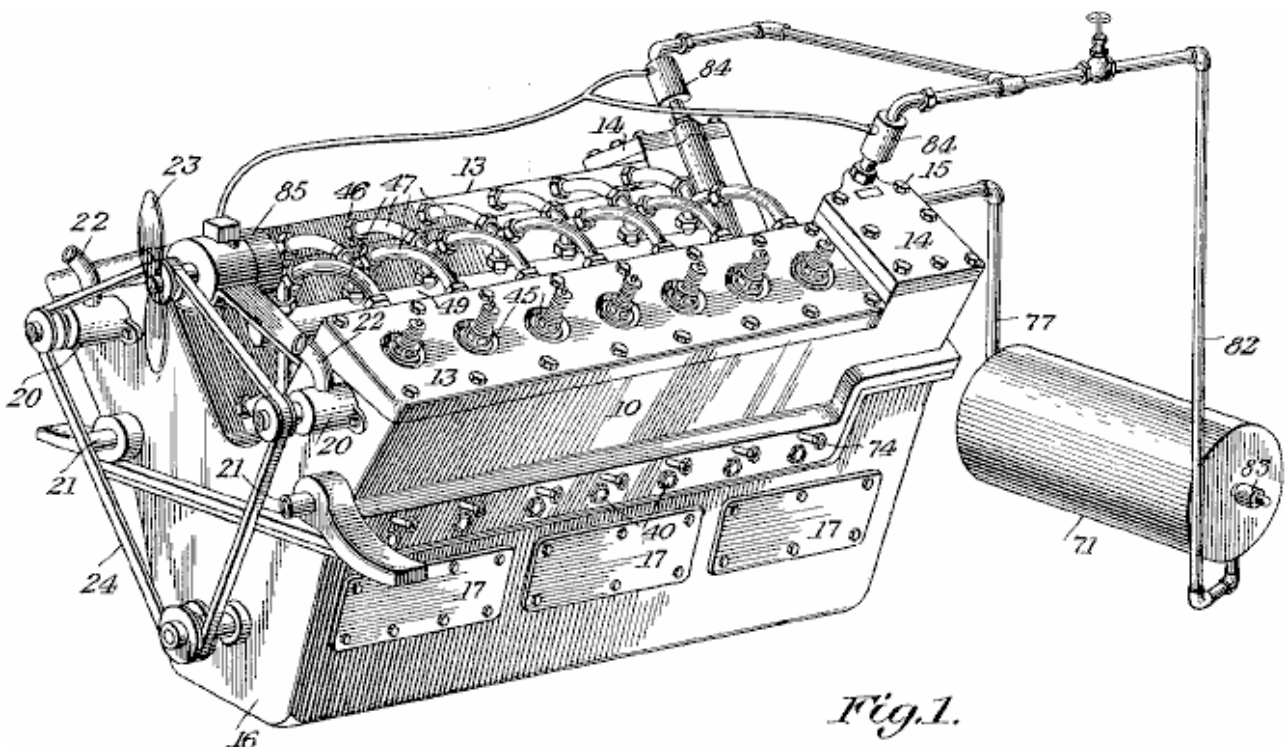
In the drawings, Fig.1 is a perspective view of the engine constructed in accordance with the invention.
