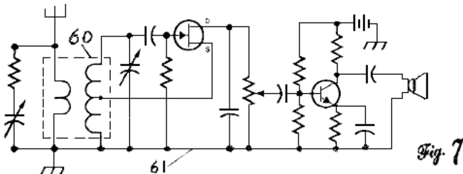
Fig.7 shows a view of a full-length transformer, used as an inductance in a radio receiver or other similar electronic circuit 61 . In this case the transmitter coil is between the aerial and ground, and the collector coil acts as the radio frequency inductance.
