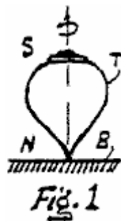
Fig.1 illustrates a magnetic spinning top, used to describe the basic principles of the invention.
