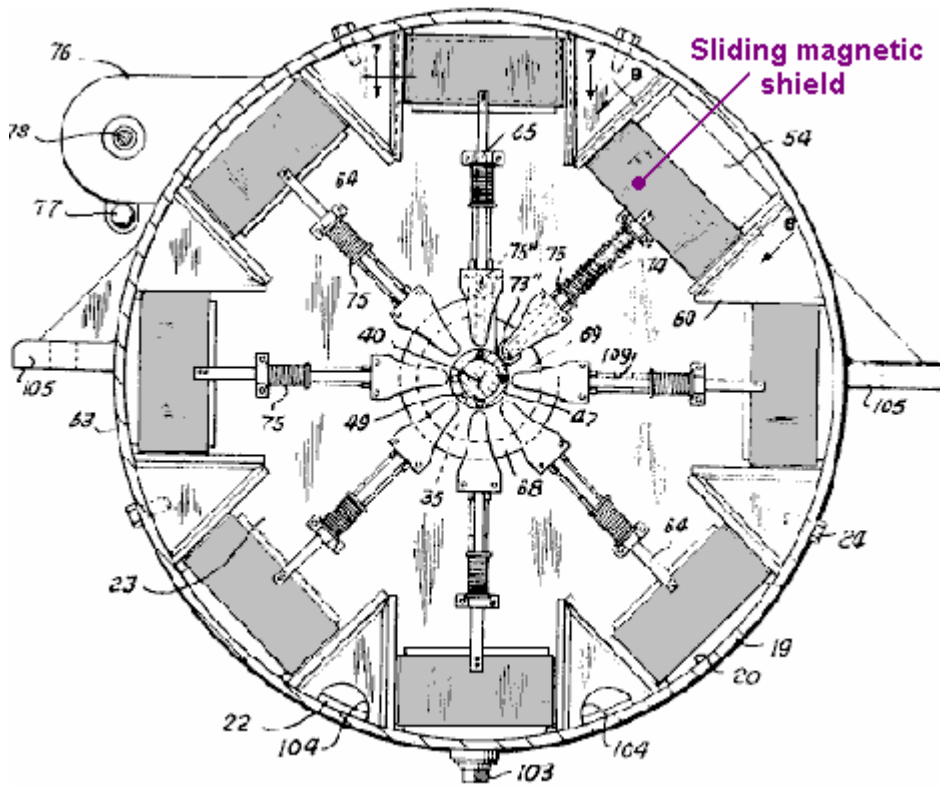
END VIEW
