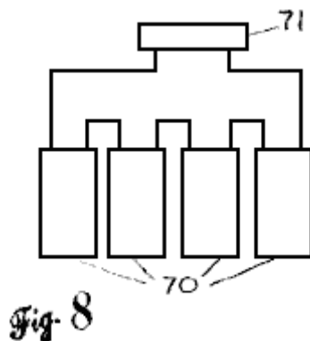
Fig.8 shows a number of full-length transformers, connected in series. They all have rectifiers to convert the high frequency AC current to DC current and the voltages at the load add up.
